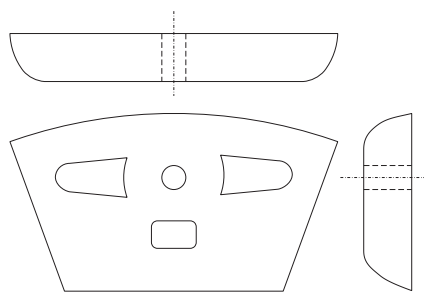
Nose Block - Make from 1/4" balsa
